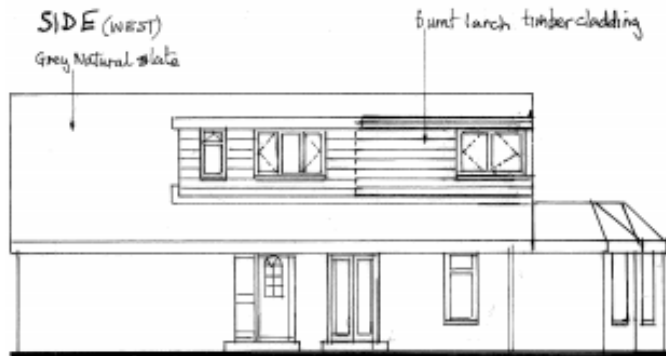
PROPOSED ELEVATIONS
